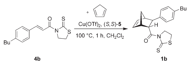
Scheme 2. The preparative DA reaction.
