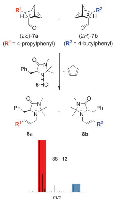
Figure 2. ESI-MS screening of organocatalysts.
