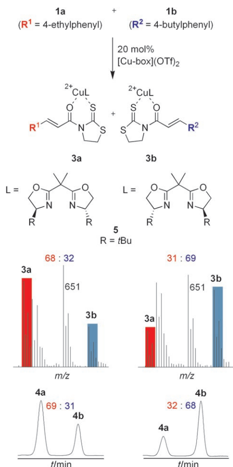
Figure 1. ESI-MS screening of the copper-catalyzed retro-DA reaction.
