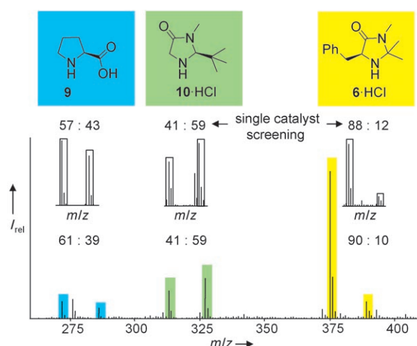
Figure 3. Simultaneous screening of three organocatalysts.
