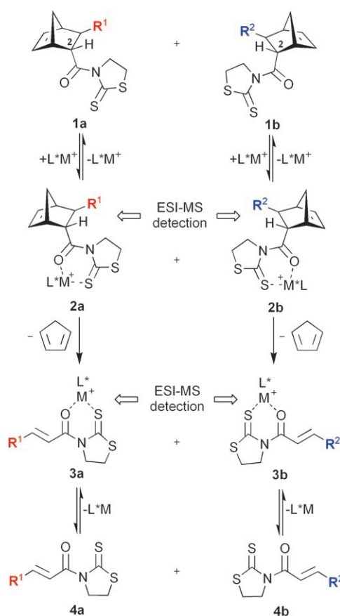
Scheme 1. Retro-Diels–Alder reaction of two quasienantiomeric Diels–Alder products 1a and 1b . R^1 and R^2 represent mass labels.
